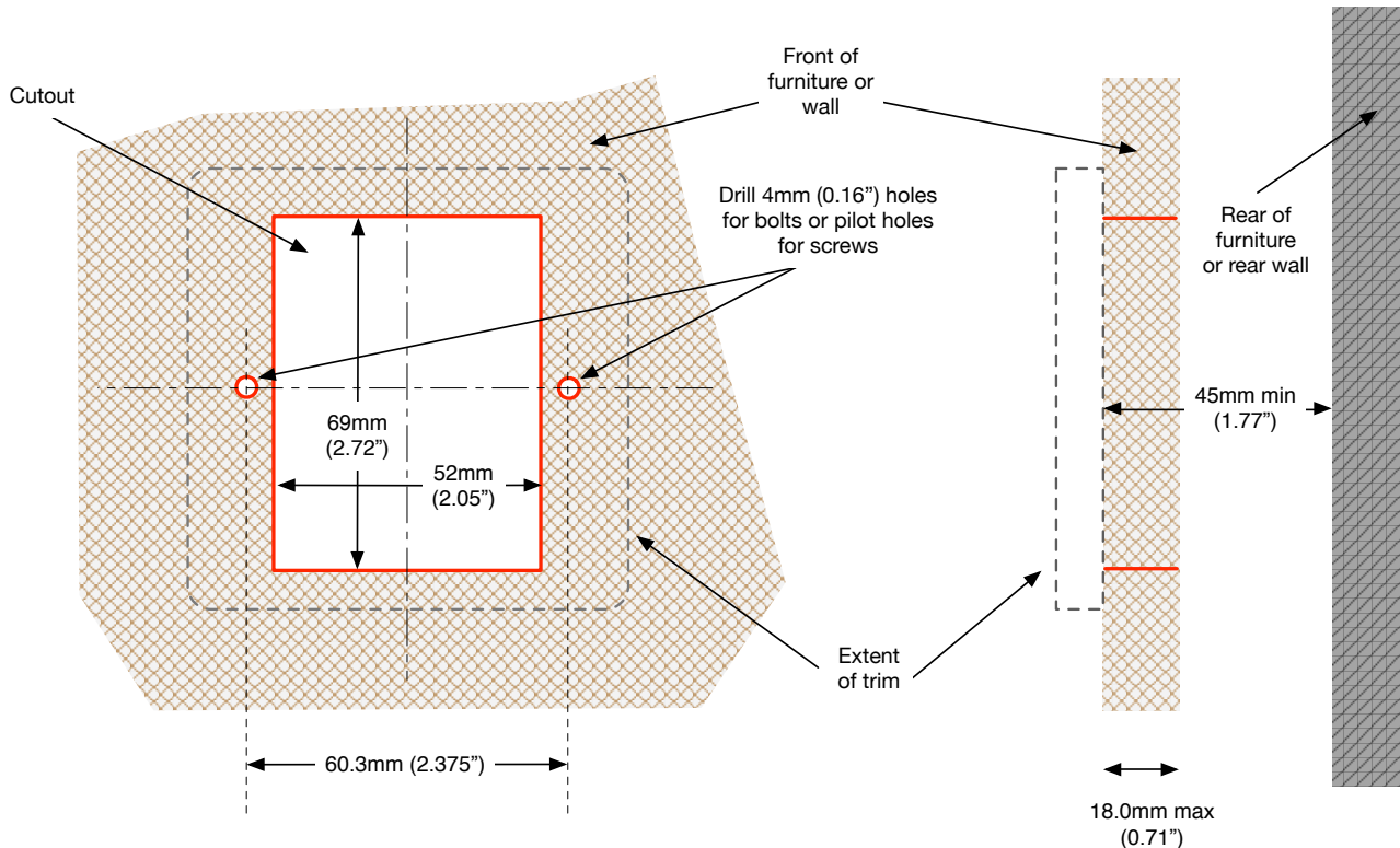
MediaHub UHD - Furniture Cutout Dimensions
